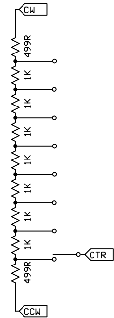
Mode Switch Wiring (X2)
