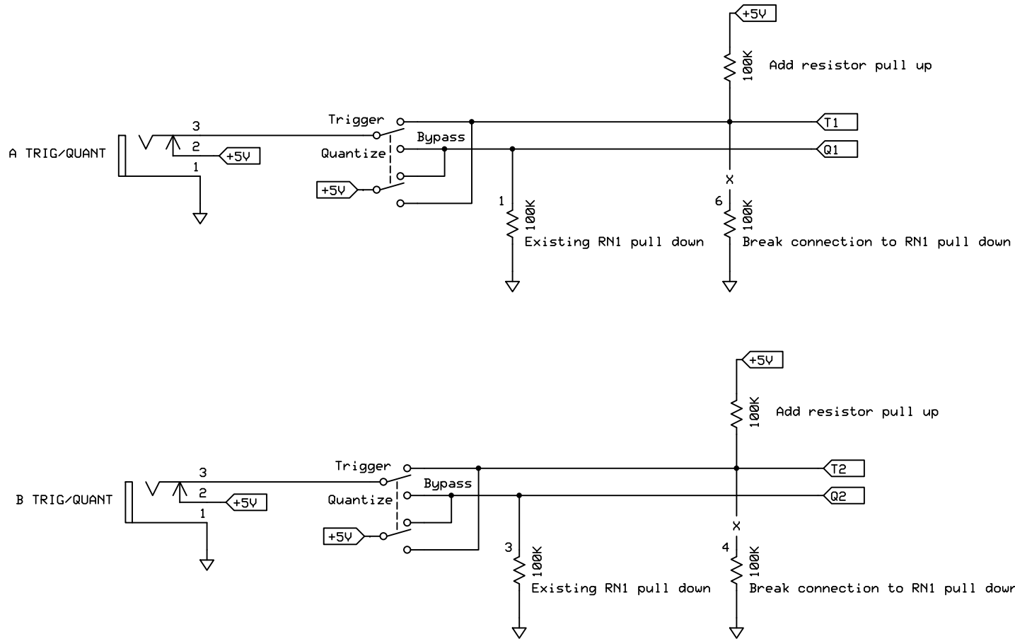
Mode Switch Wiring (X2)
